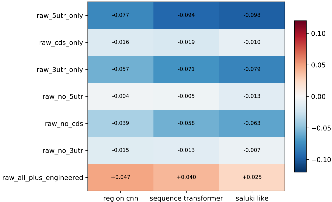
Mean chromosome-holdout Pearson delta versus raw all
