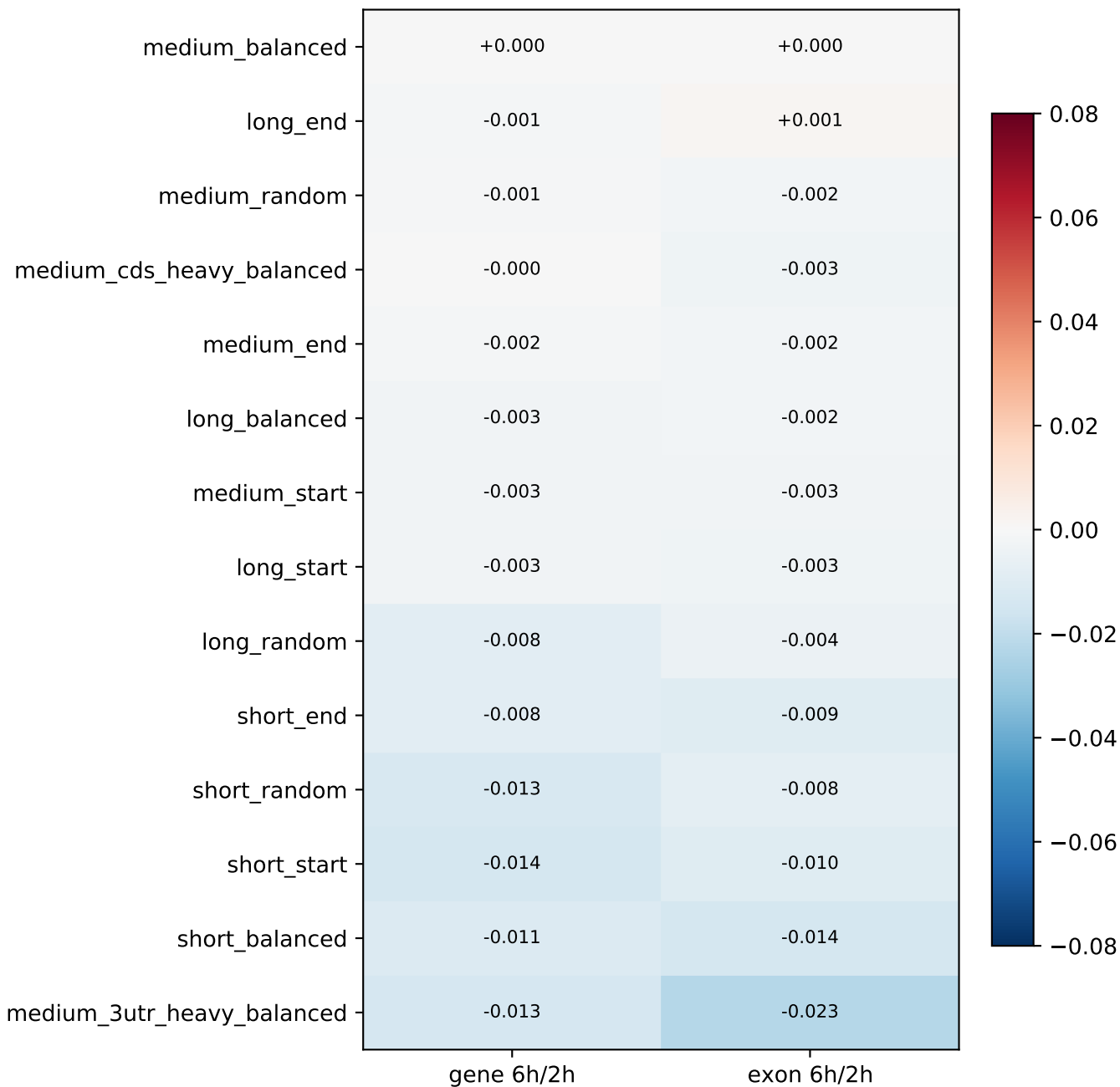
Paired Pearson delta versus medium balanced
