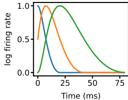
Pillow basis for g_{i \rightarrow j}
