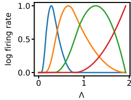
basis for f_{damp}(\Lambda)
