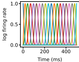
B-spline basis for f_j(t)
