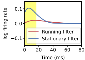
Illustration of excursion statistics
