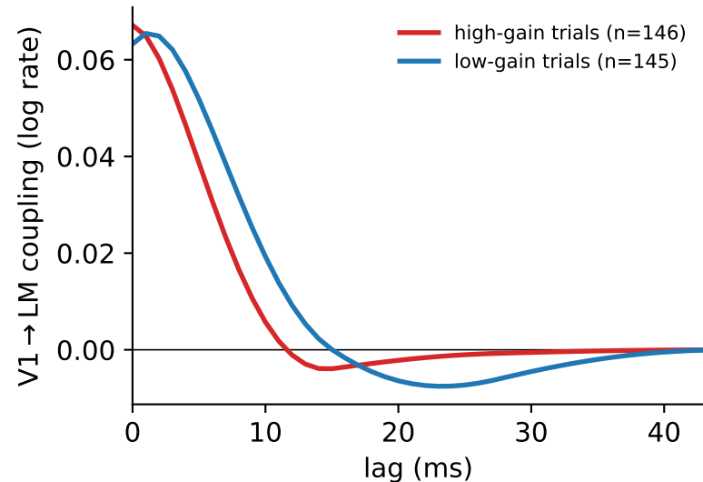
A V1 \rightarrow LM coupling by trial gain (session 757216464, running trials)
