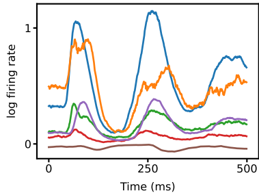
Population firing rate components predicted by GLM
