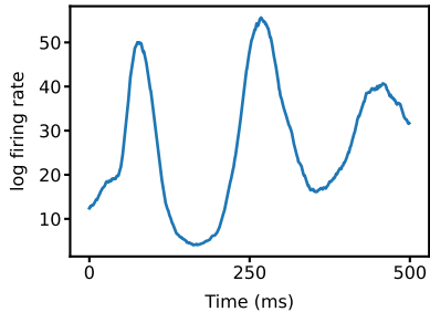
EIF neuron firing rate
