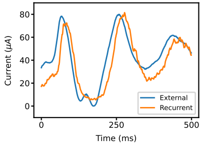
Input current to EIF neurons
