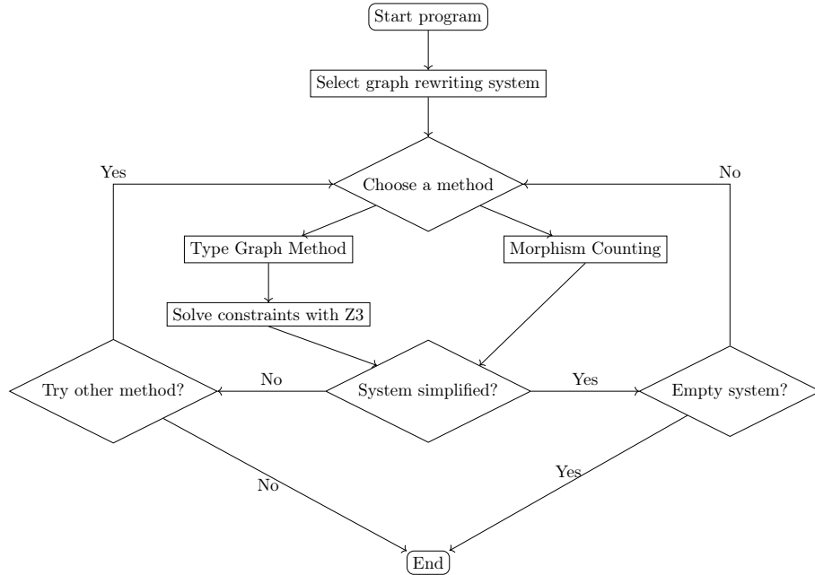
Figure 1: Workflow of LyonParallel
