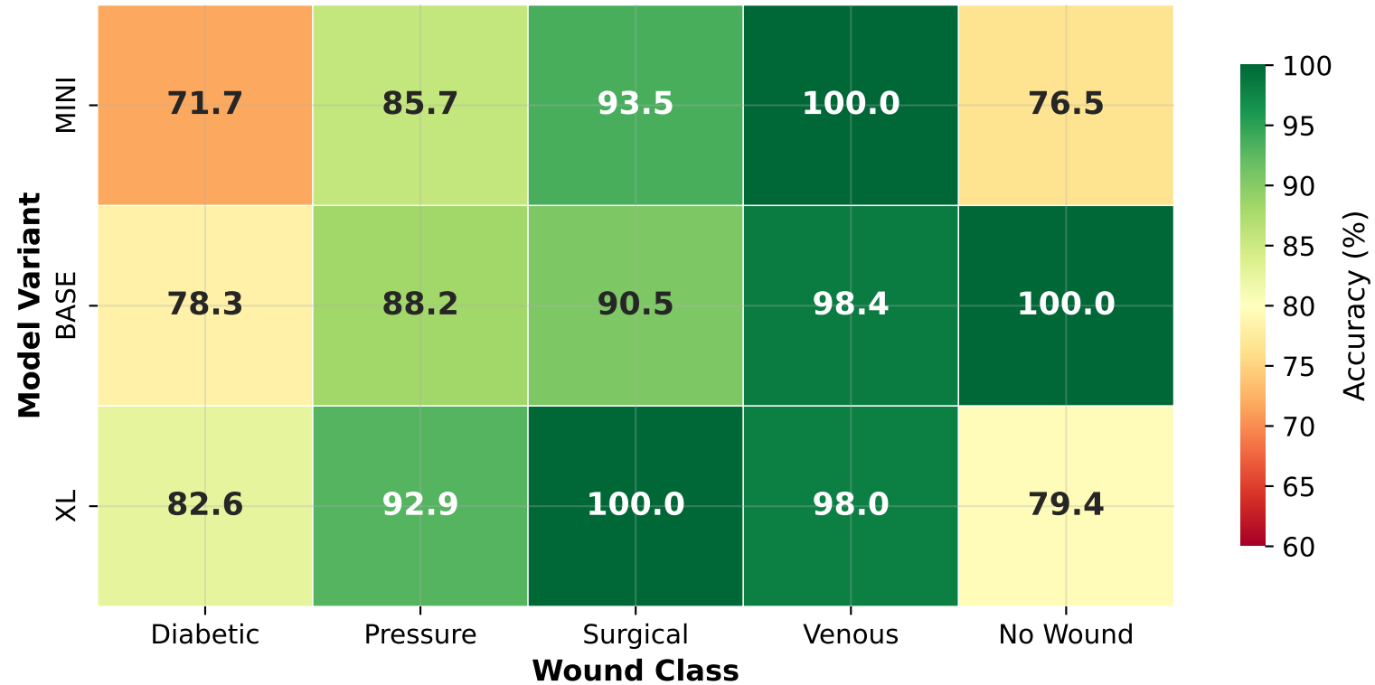
Per-Class Classification Accuracy (%)
