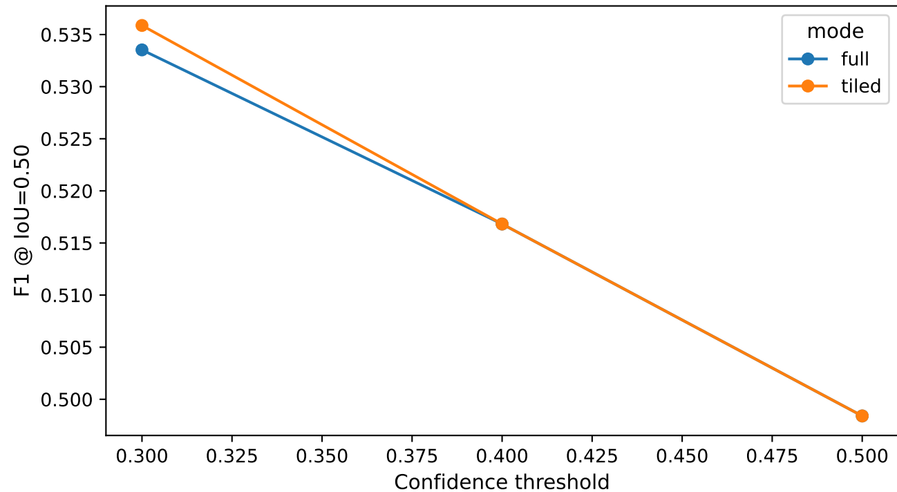
Full vs tiled evaluation: F1@IoU50 vs confidence
