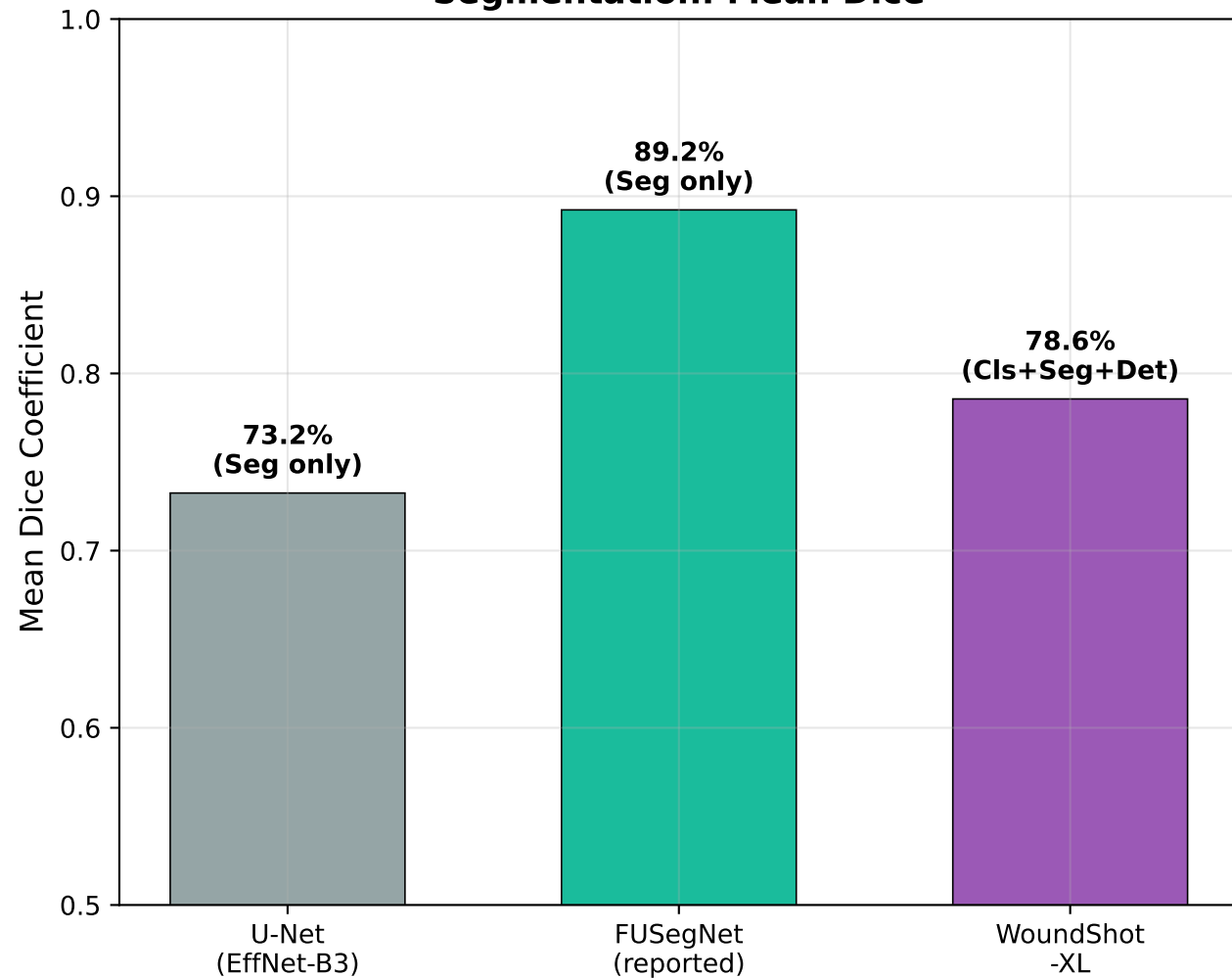
Segmentation: Mean Dice
