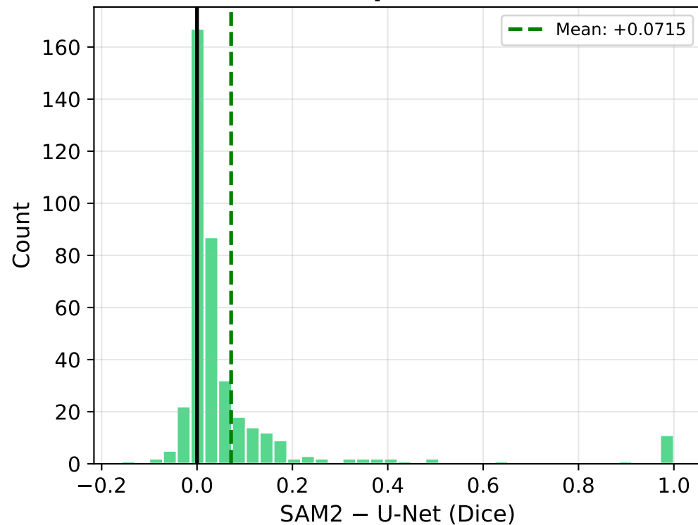
SAM2 vs U-Net Wilcoxon: p=1.28e-36 ★
