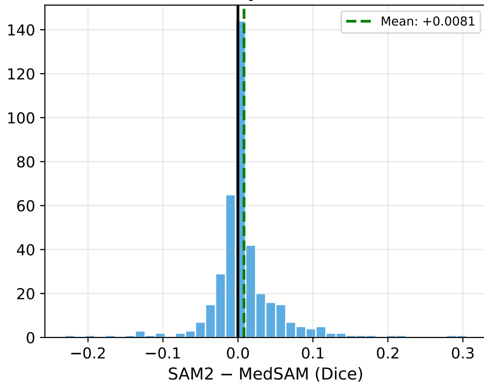
SAM2 vs MedSAM Wilcoxon: p=2.91e-04 ★
