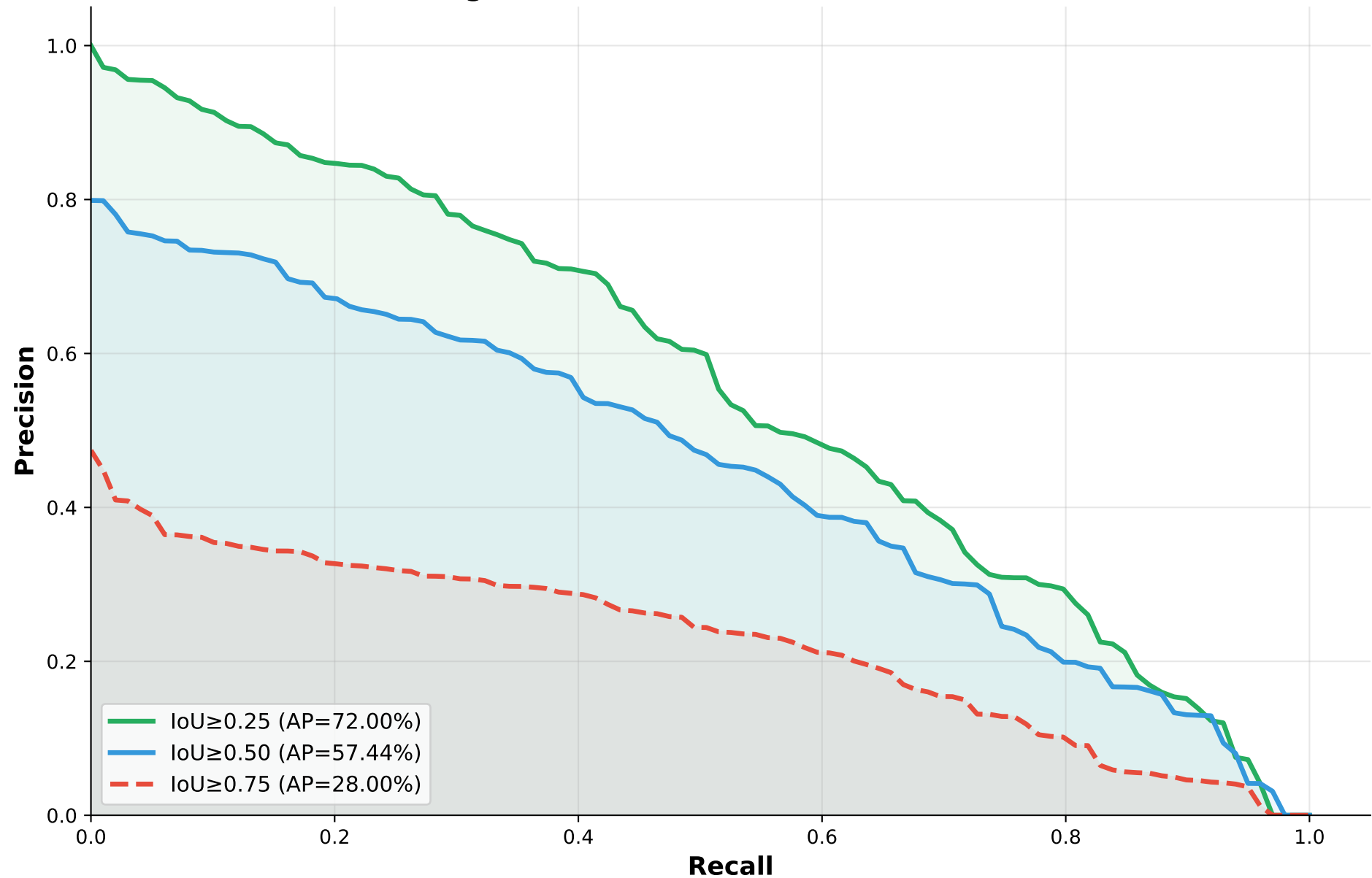
Seg→Det Precision-Recall Curve at Multiple IoU Thresholds Strong Performance at \text{IoU} \geq 0.25 and \text{IoU} \geq 0.5
