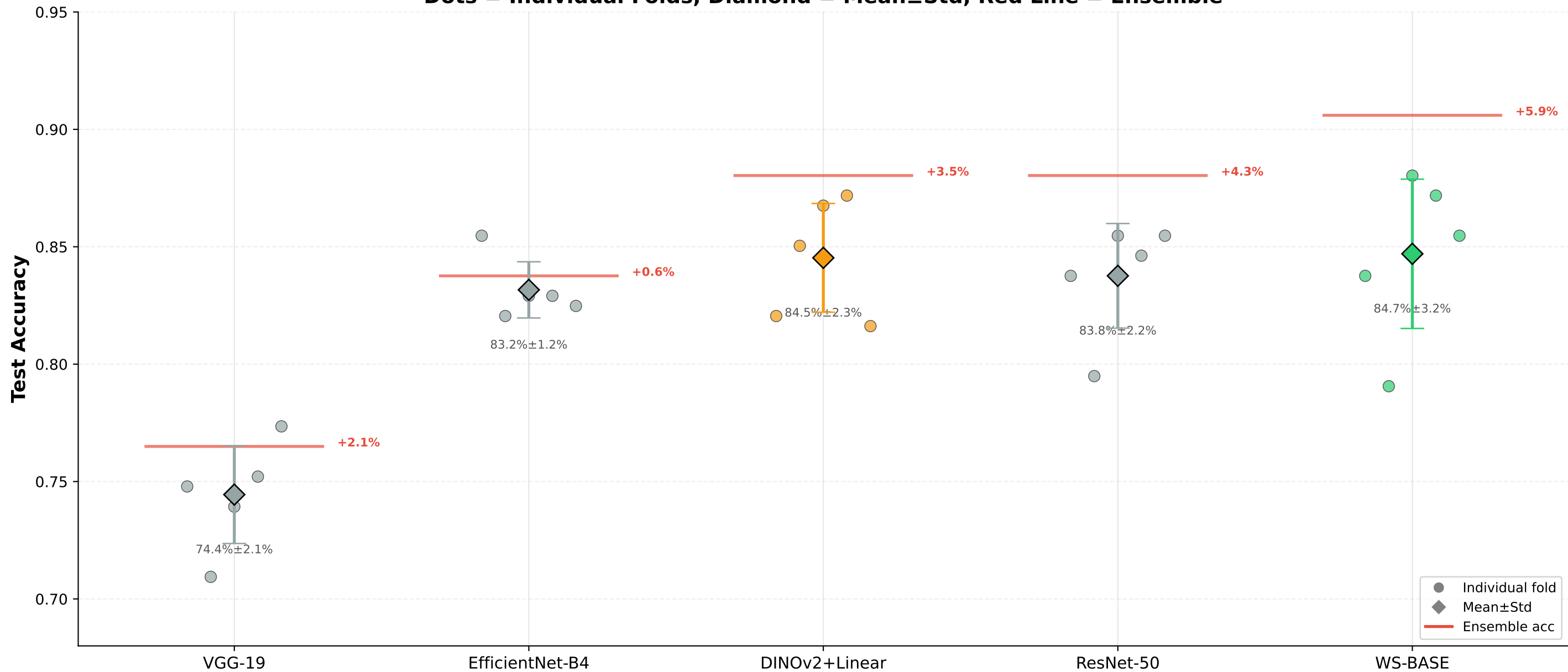
Per-Fold Accuracy with Ensemble Gain Dots = Individual Folds, Diamond = Mean \pm Std, Red Line = Ensemble
