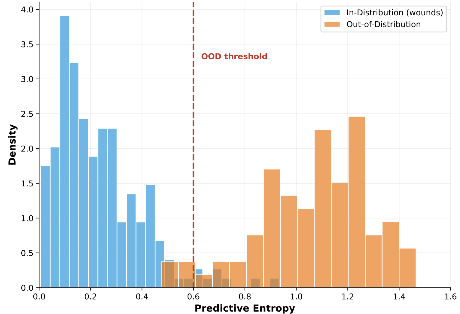
In-Distribution vs OOD Detection High Entropy Flags Unknown Inputs
