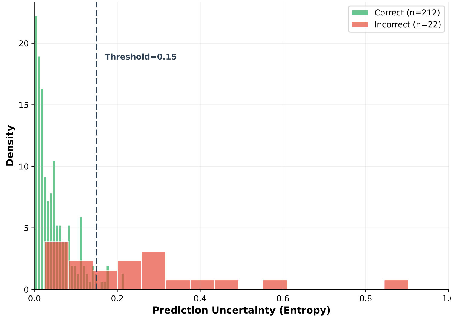
Uncertainty: Correct vs Incorrect Clear Separation Enables Error Detection
