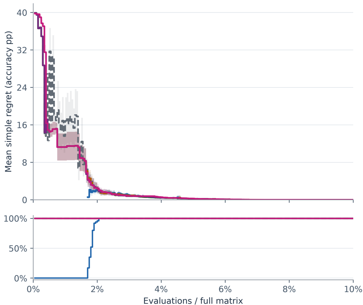
Default prior
