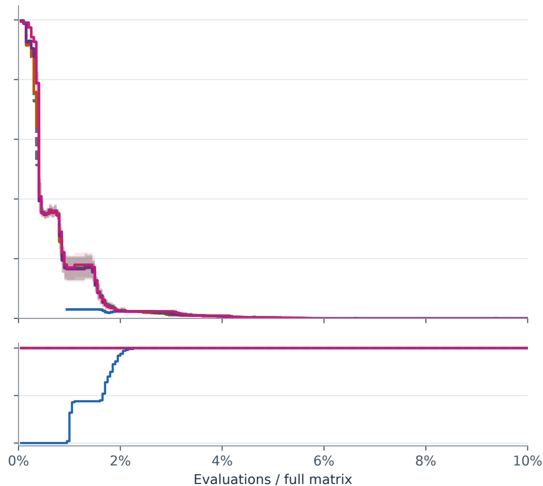
Dataset prior
