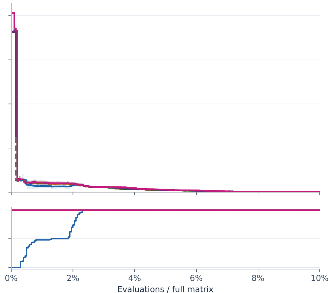
Dataset prior: N(0.4, 0.02)
