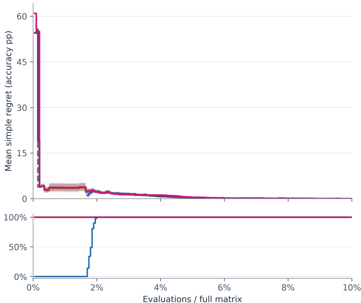
Default prior: N(0.5, 0.04)
