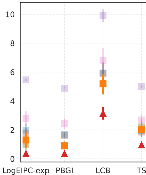
Higgs
