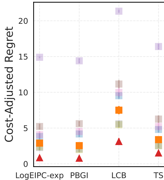
Fashion-MNIST
