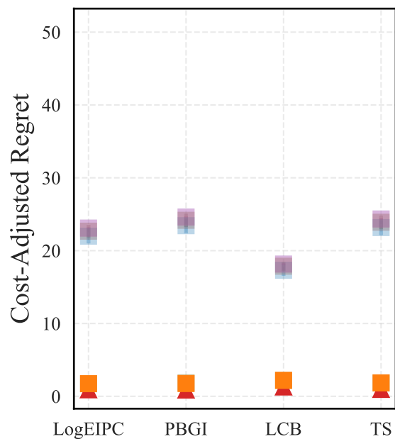
cifar10-valid
