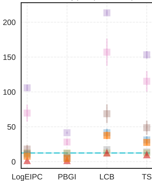
Covertypes (581012)
