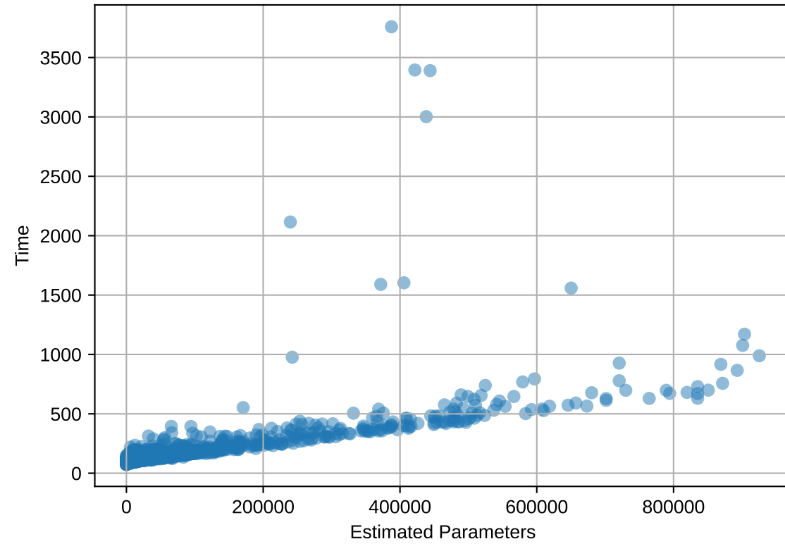
bank-marketing: Time vs Estimated Params
