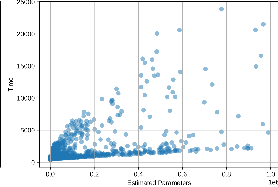
car: Time vs Estimated Params
