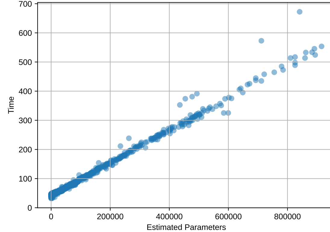
blood-transfusion-service-center: Time vs Estimated Params
