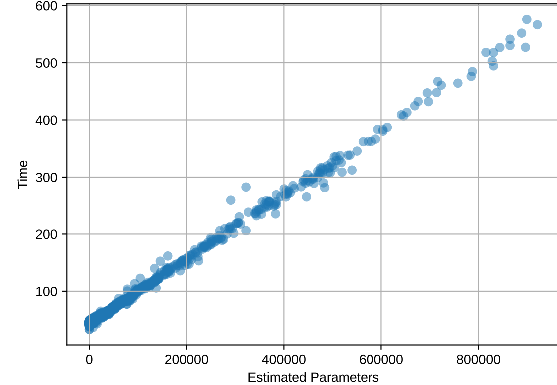
car: Time vs Estimated Params
