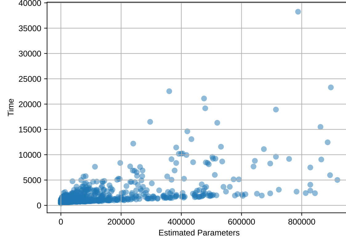
blood-transfusion-service-center: Time vs Estimated Params
