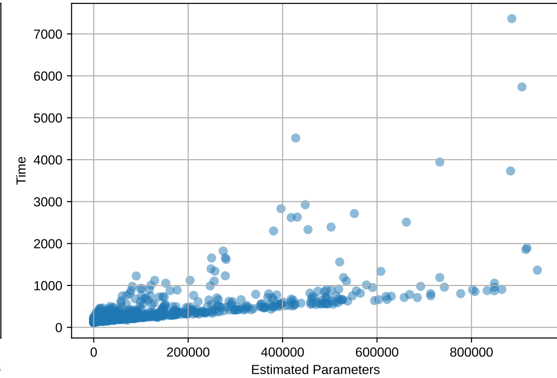
jungle_chess_2pcs_raw_endgame_complete: Time vs Estimated Params
