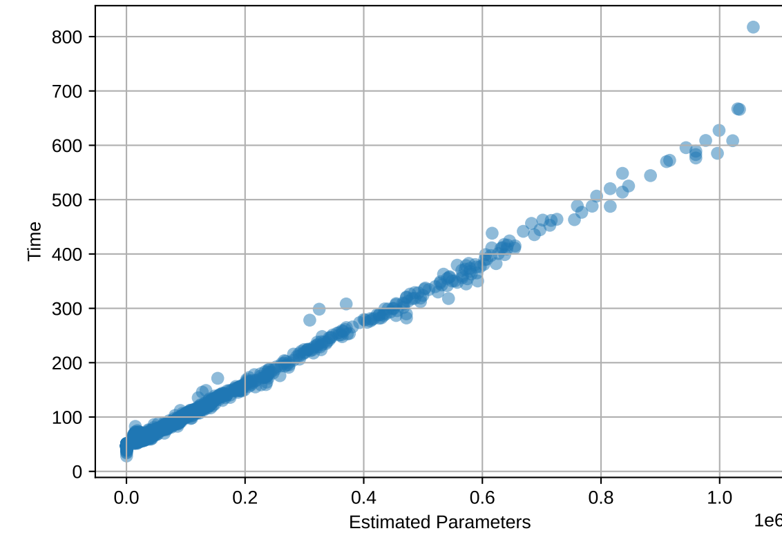
jasmine: Time vs Estimated Params
