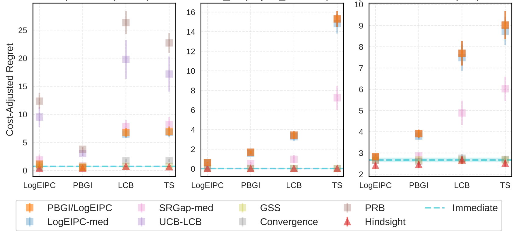
Apsfailure (76000)
