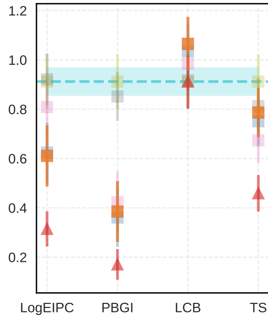
Mfeat-factors (2000)
