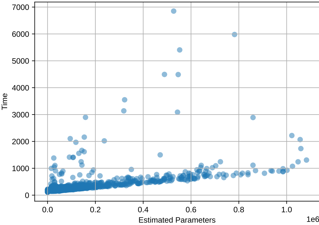
Fashion-MNIST: Time vs Estimated Params
