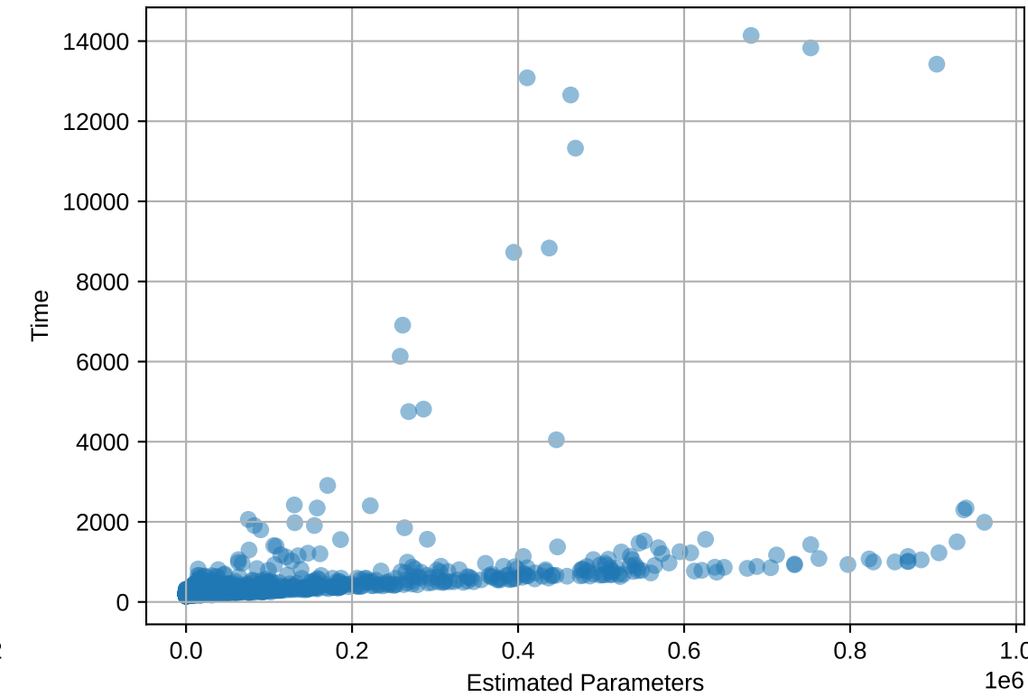
MiniBooNE: Time vs Estimated Params
