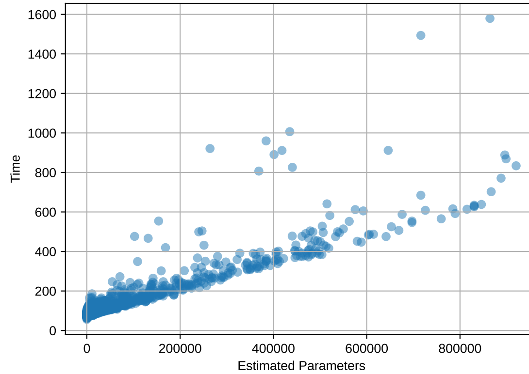
KDDCup09_appetency: Time vs Estimated Params
