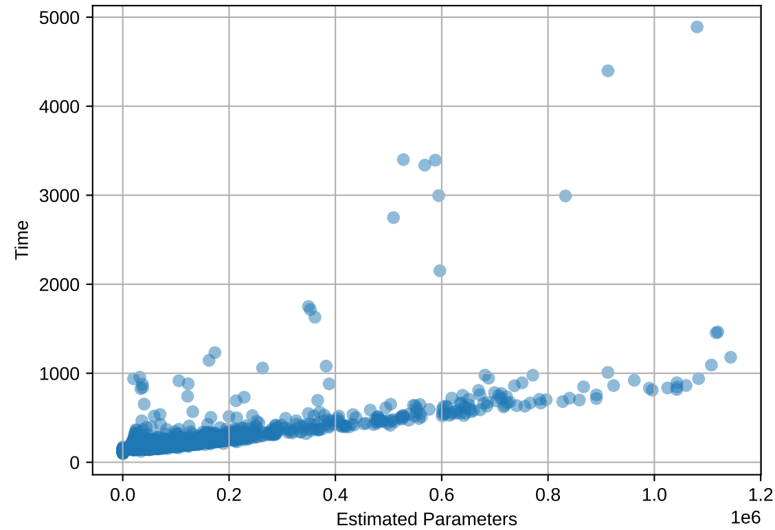
KDDCup09_appetency: Time vs Estimated Params
