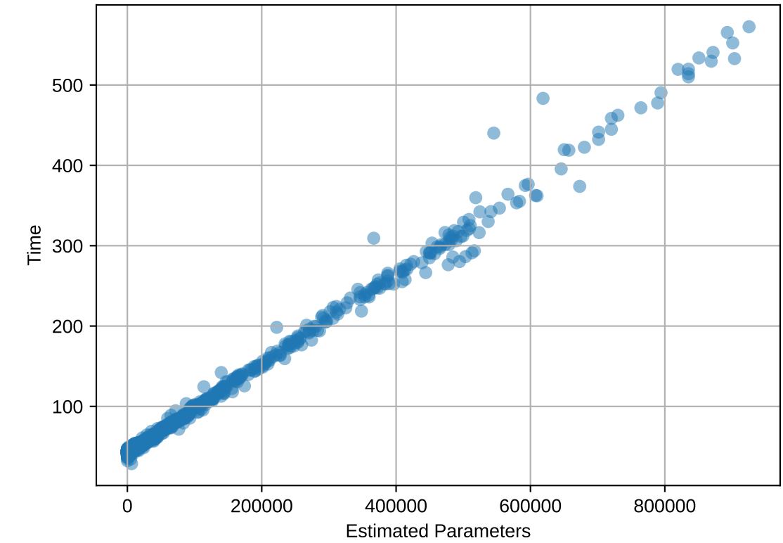
MiniBooNE: Time vs Estimated Params
