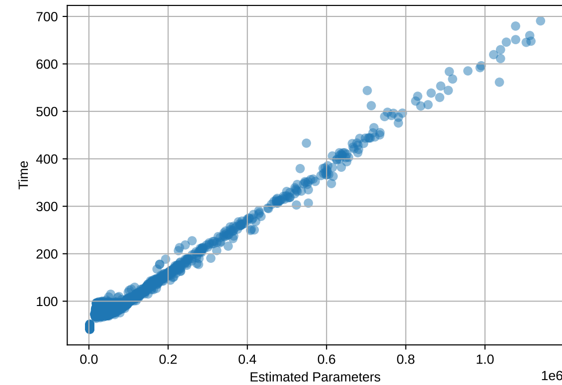
phoneme: Time vs Estimated Params
