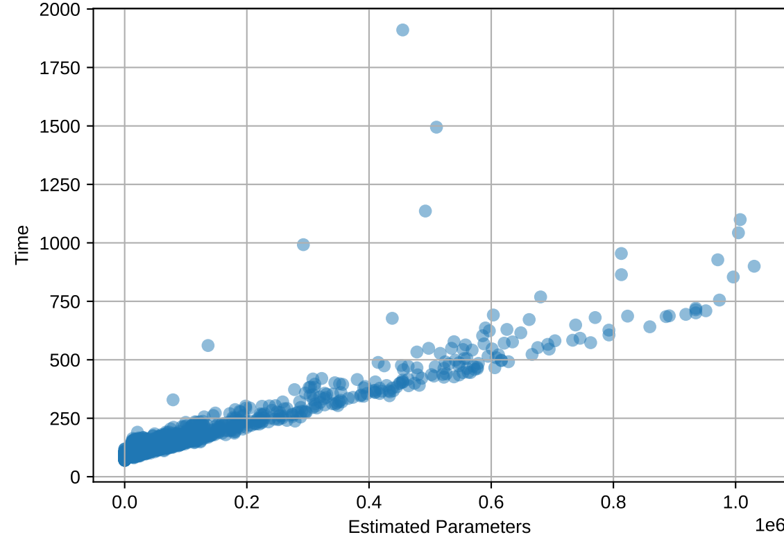
nomao: Time vs Estimated Params
