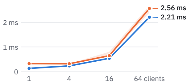
80 % reads, 20 % writes: 95th percentile latency
