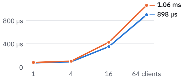
Reads: 95th percentile latency
