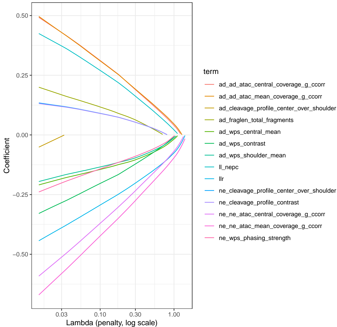
Coefficient paths of top features
