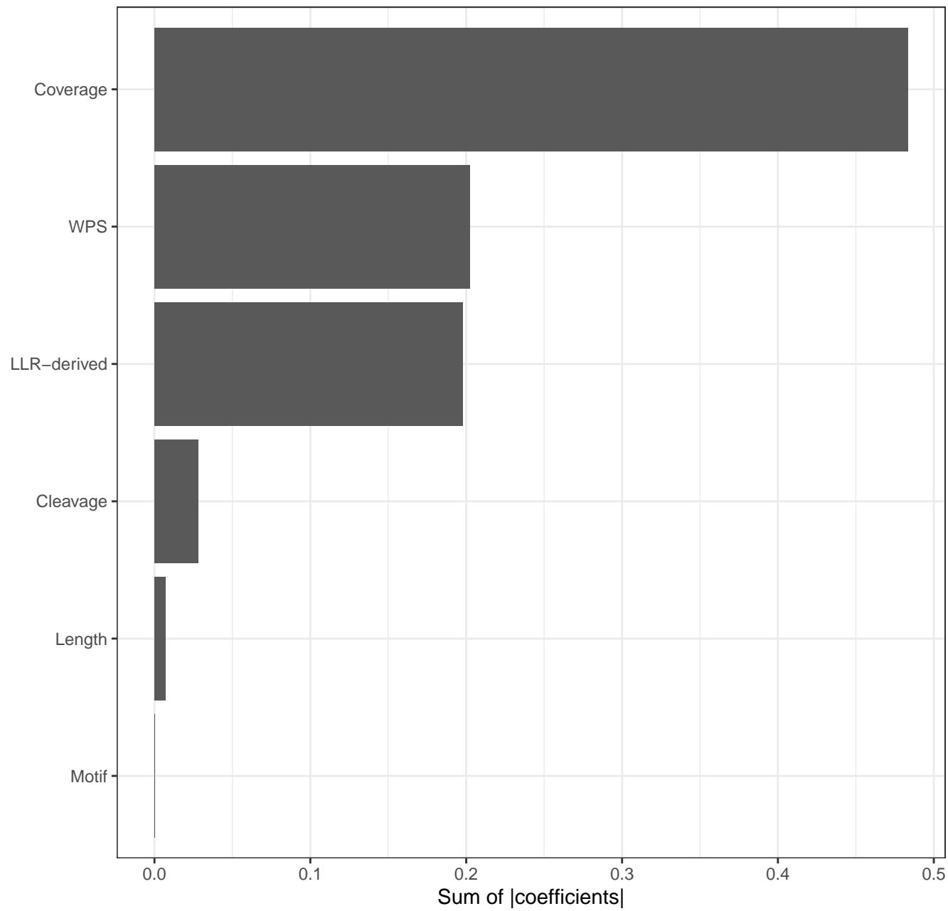
Family-level importance (glmnet coefficients)
