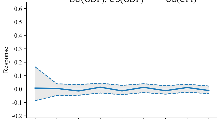
(a2) The time-invariant OIRF
