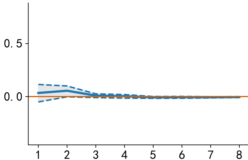
EU (GDP) → US (GDP)
