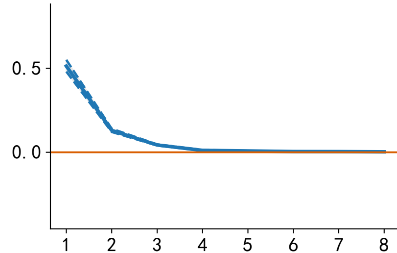
US (CPI) → US (CPI)
