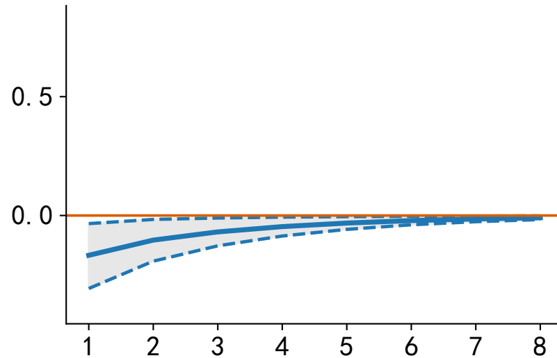
EU (GDP) → US (HUR)
