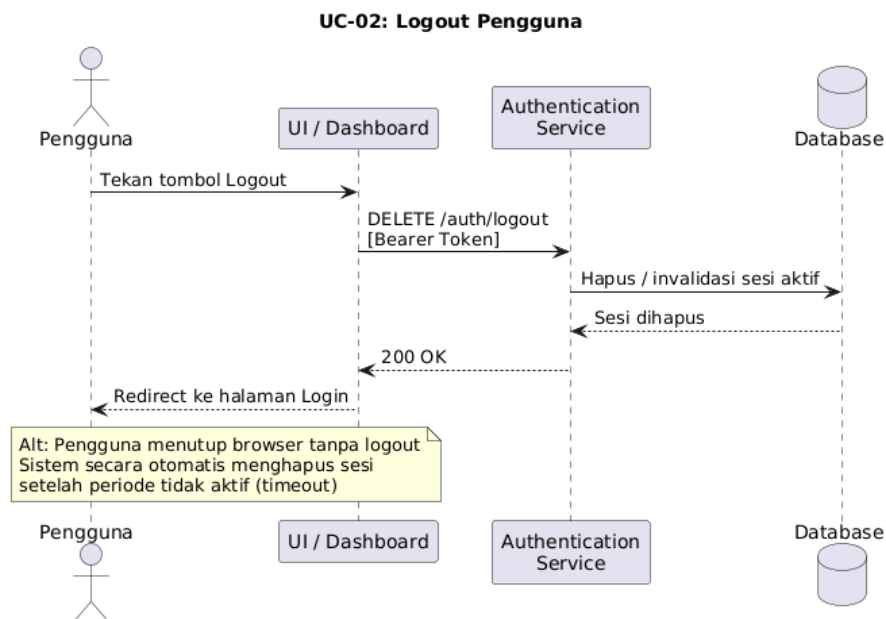
Gambar IV.16 Diagram sequence UC-02: Logout Pengguna
