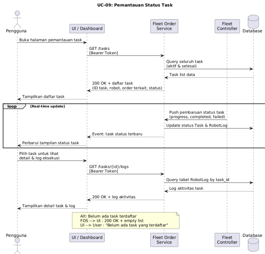
Gambar IV.23 Diagram sequence UC-09: Pemantauan Status Task
