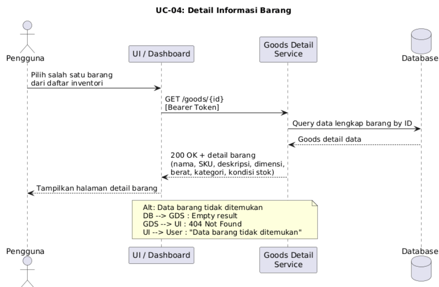
Gambar IV.18 Diagram sequence UC-04: Detail Informasi Barang
