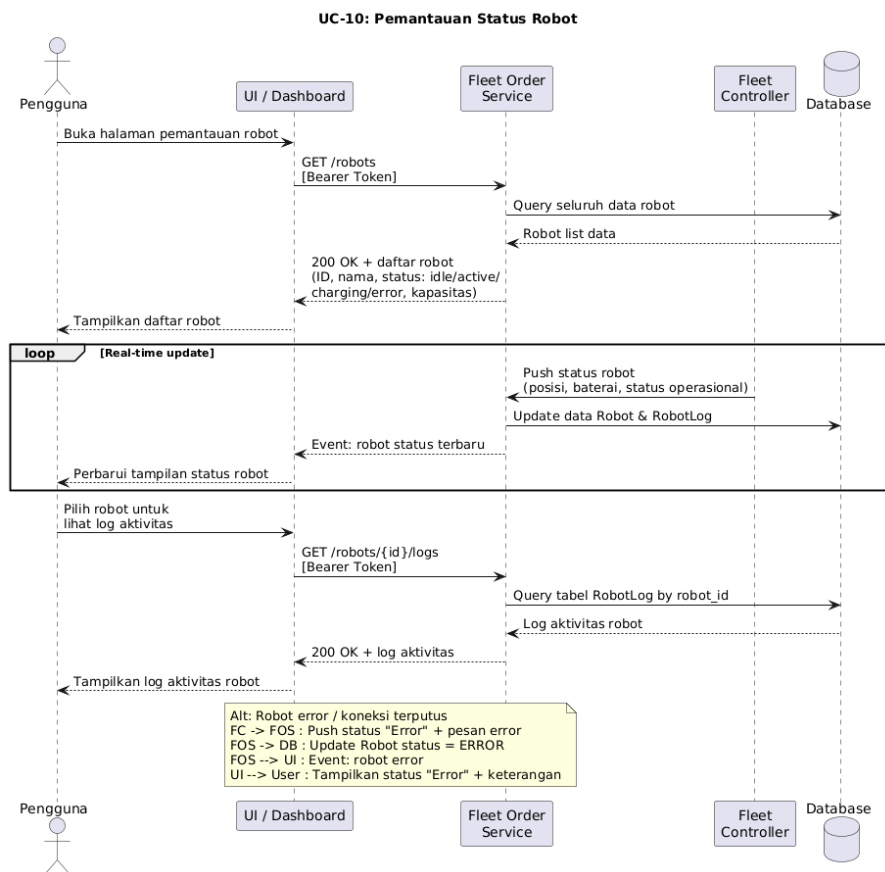
Gambar IV.24 Diagram sequence UC-10: Pemantauan Status Robot
