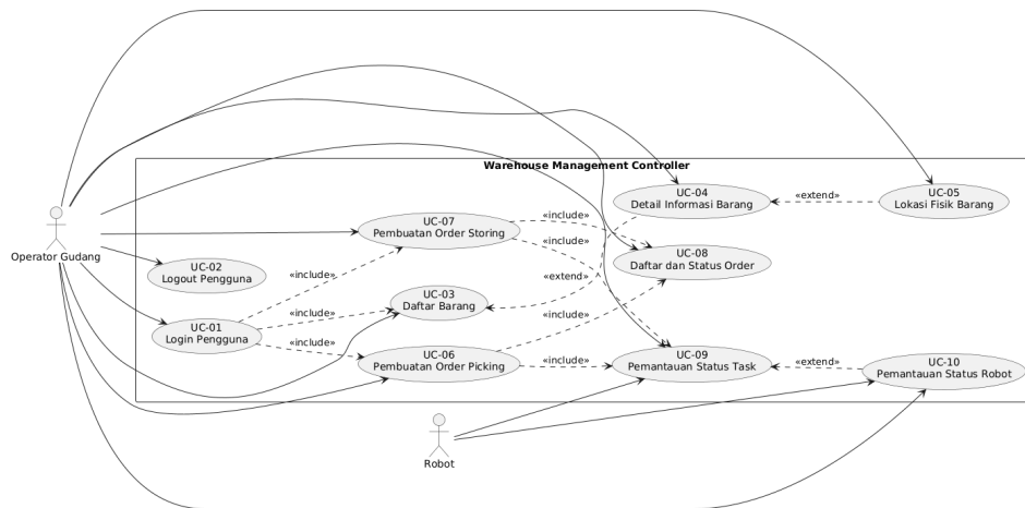
Gambar IV.14 Diagram use case sistem Warehouse Management Controller
