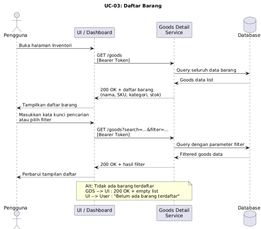
Gambar IV.17 Diagram sequence UC-03: Daftar Barang
