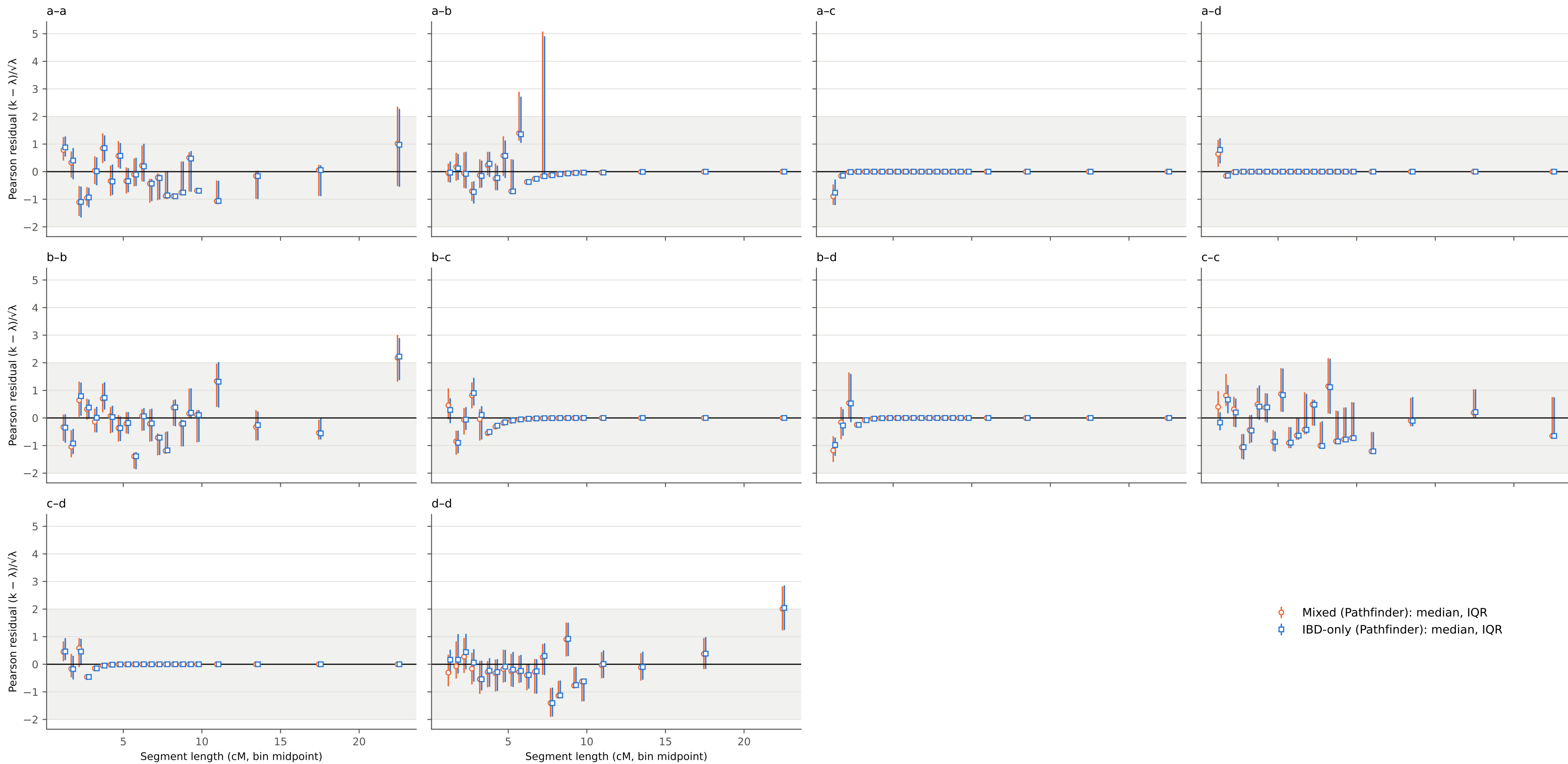
Residuals at 1000 cM, T true , hap-IBD, all 100 subsamples (grey band: \pm 2 )
