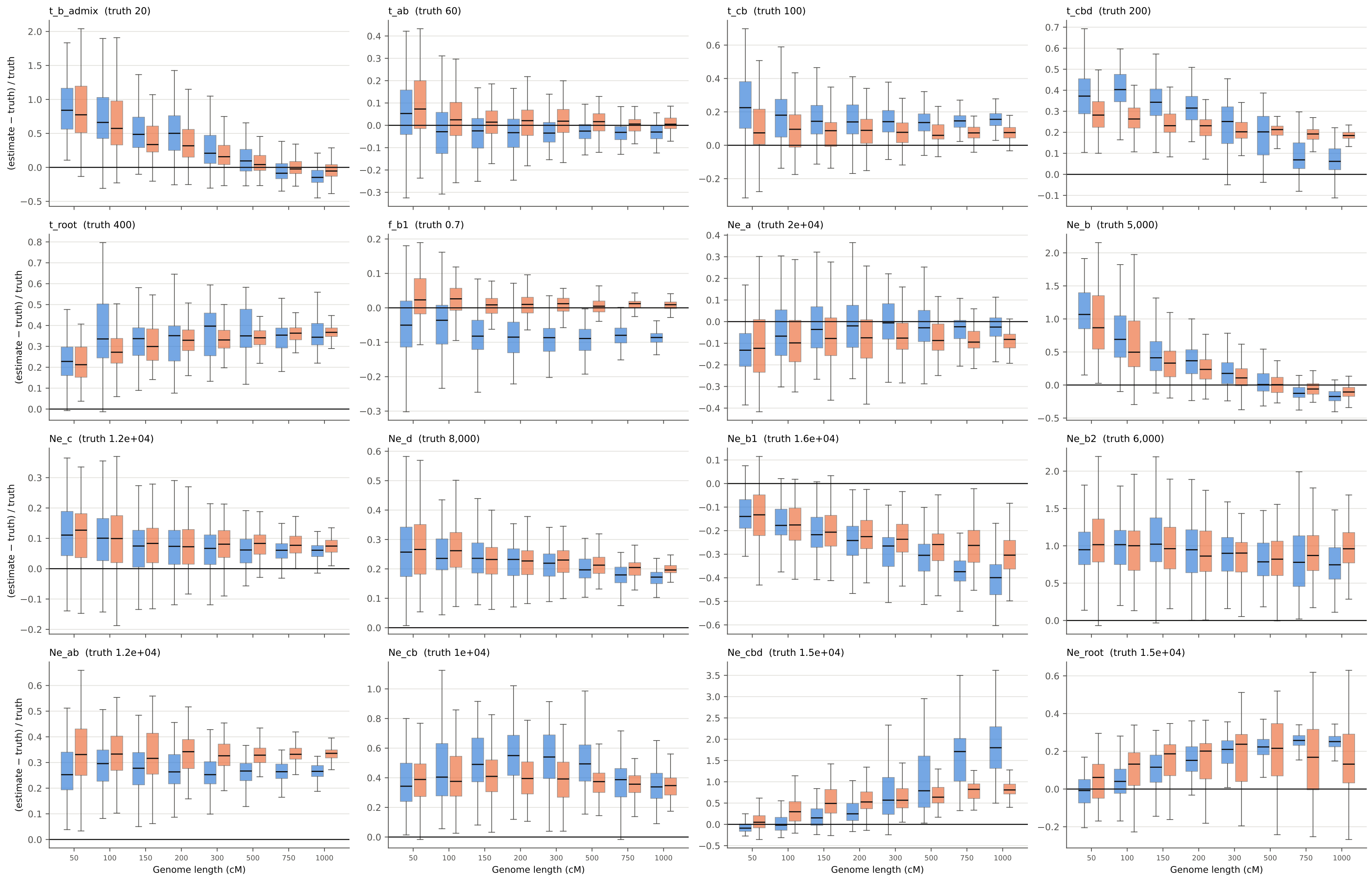
T_true parameter recovery from hap-IBD: posterior means per subsample (Ne haploid)
