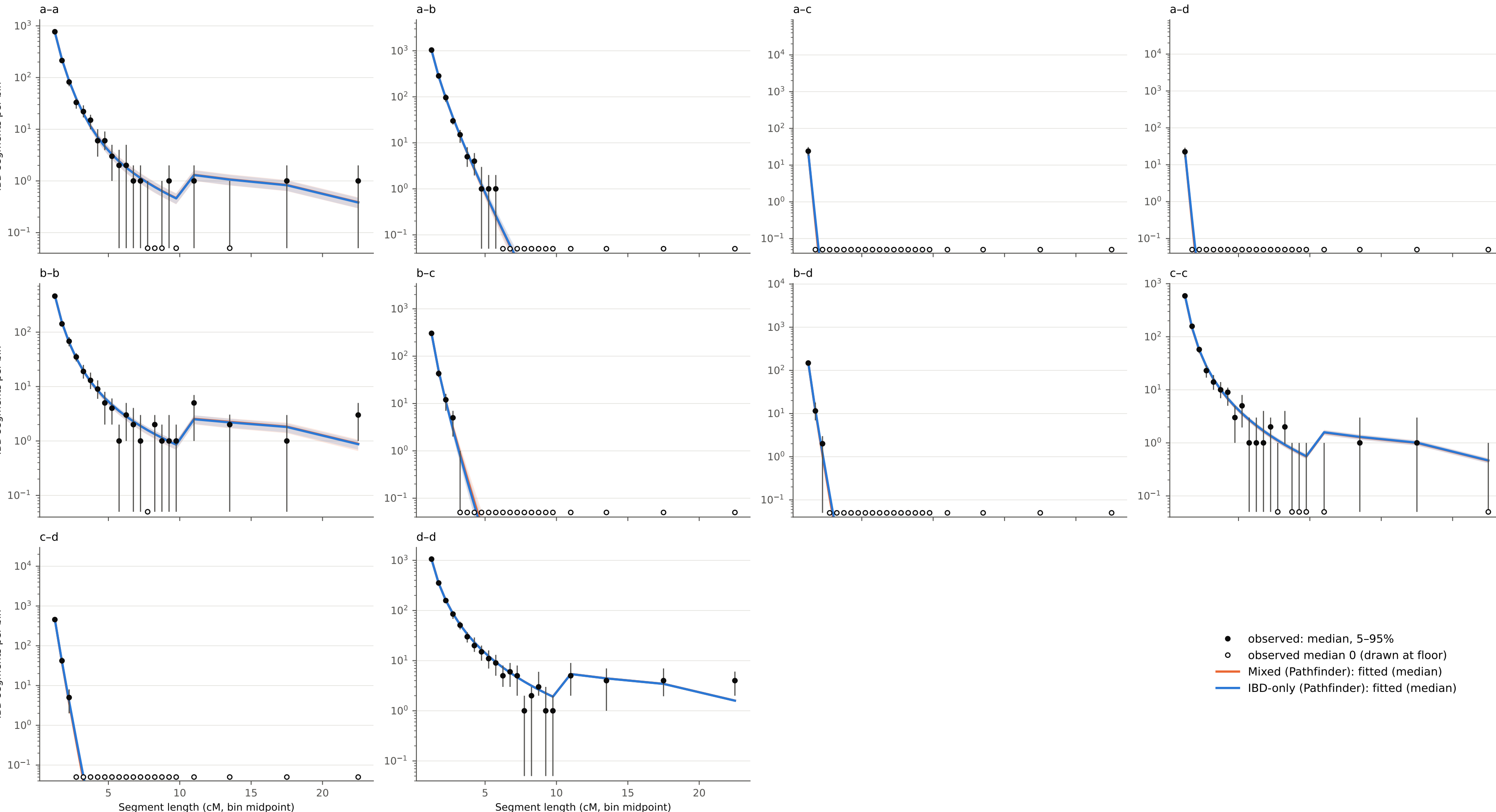
Spectrum fit at 1000 cM, T_true: every bin, all 100 subsamples (bands: 5-95% across subsamples; axis floored at 0.05 segments)
