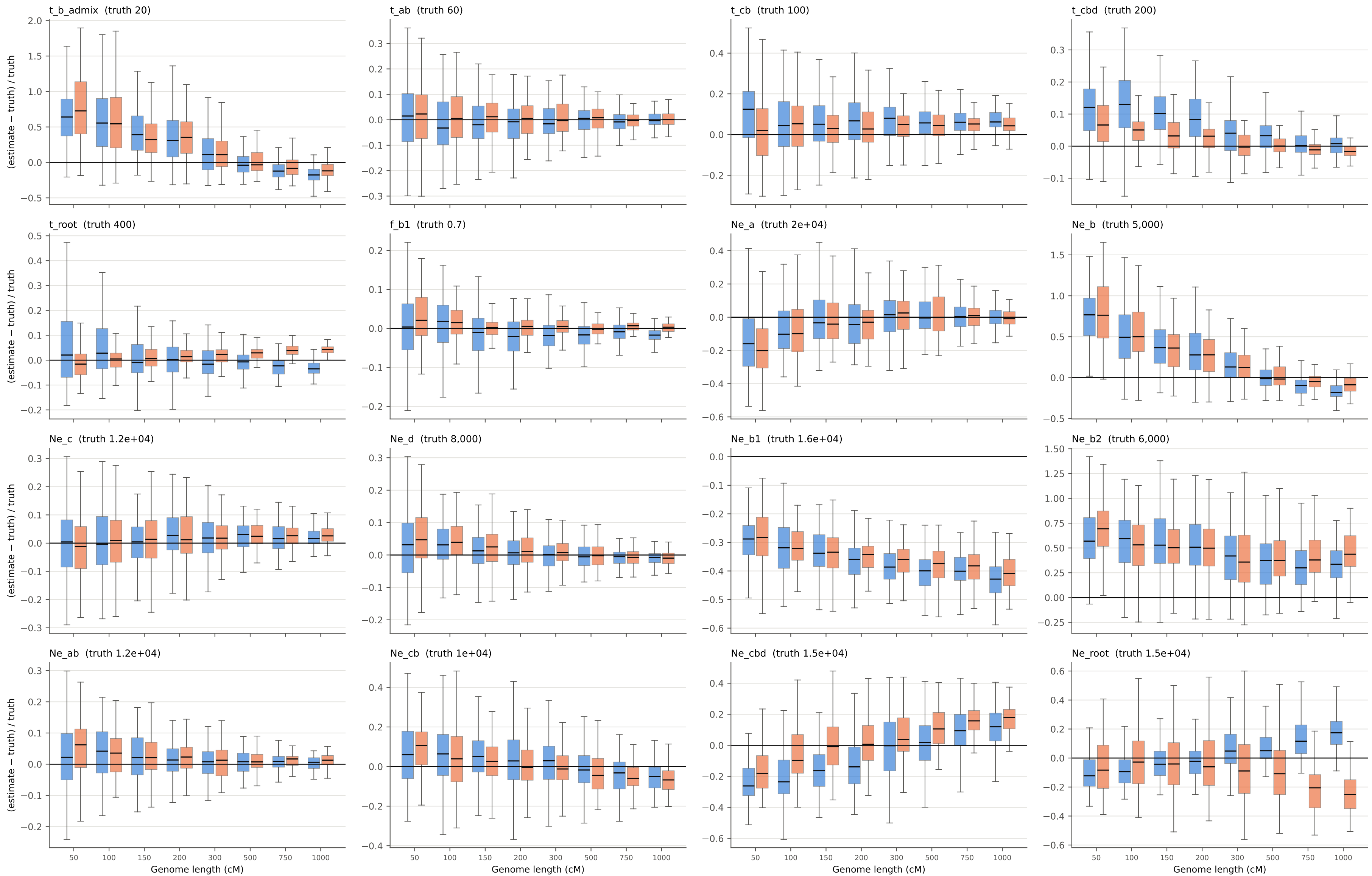
T_true parameter recovery from true IBD: posterior means per subsample (Ne haploid)
