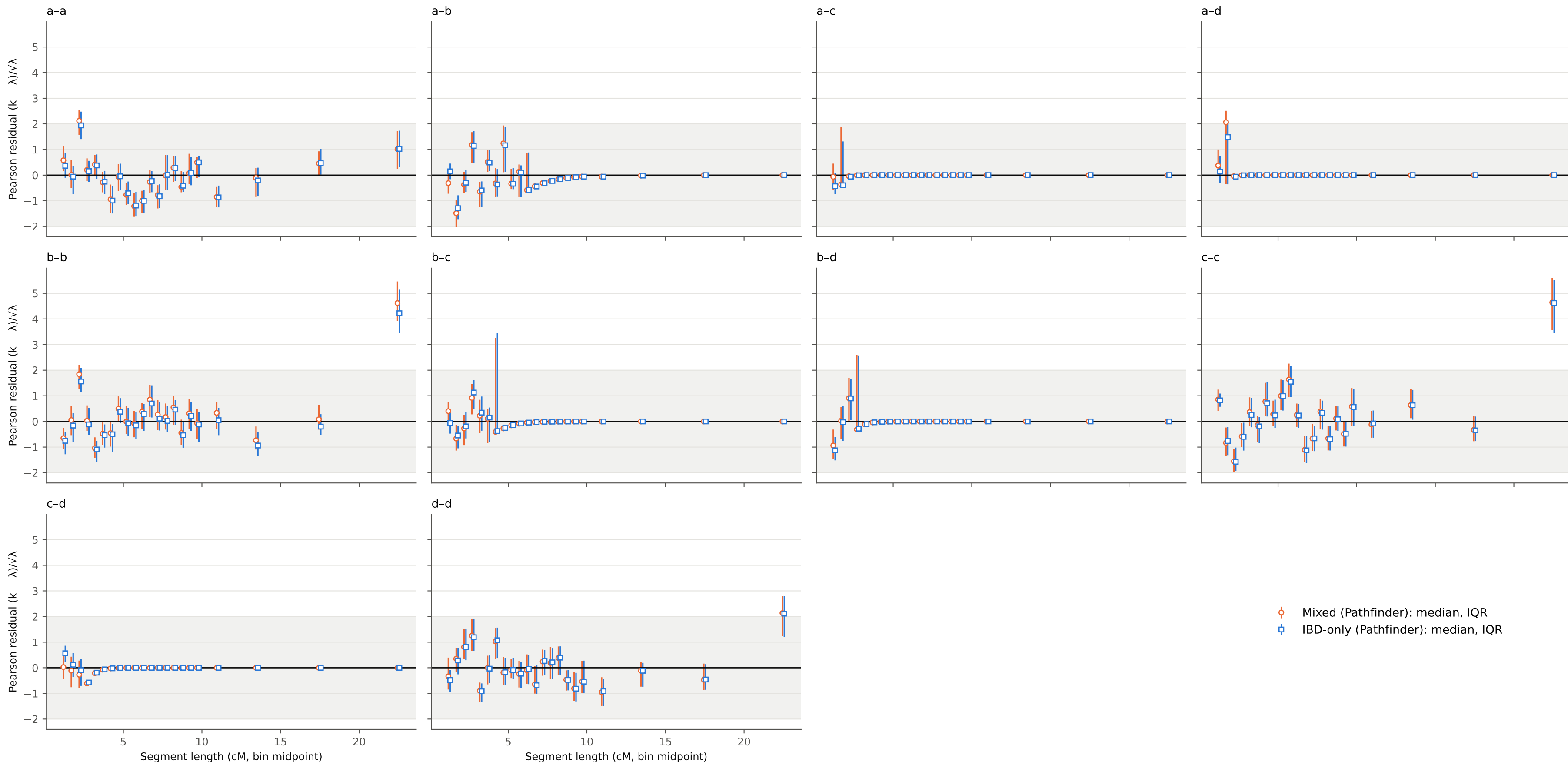
Residuals at 1000 cM, T true , true IBD, all 100 subsamples (grey band: \pm 2 )
