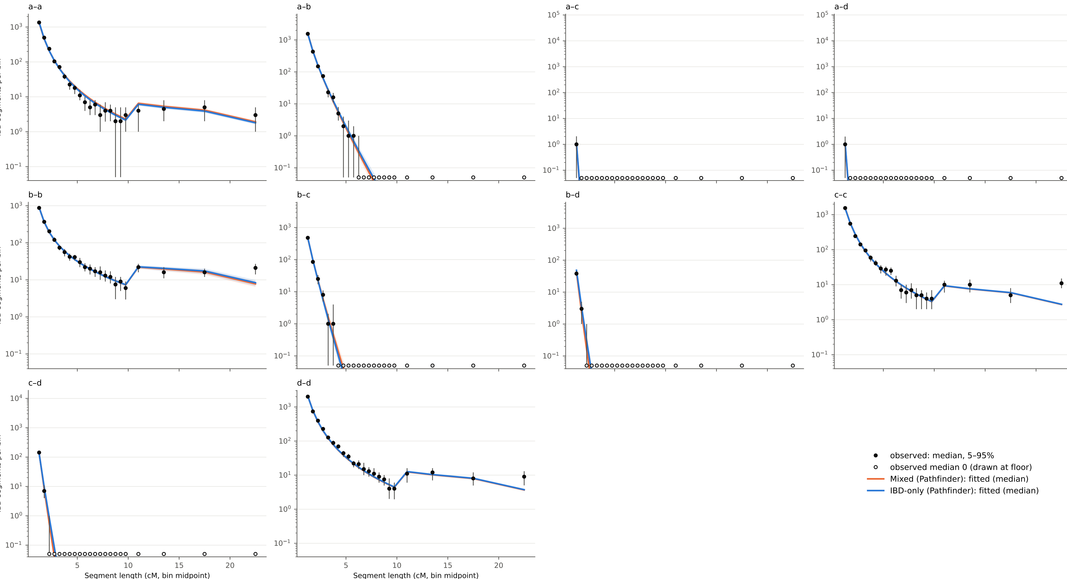
Spectrum fit at 1000 cM, T true , hap-IBD: every bin, all 100 subsamples (bands: 5-95% across subsamples; axis floored at 0.05 segments)
