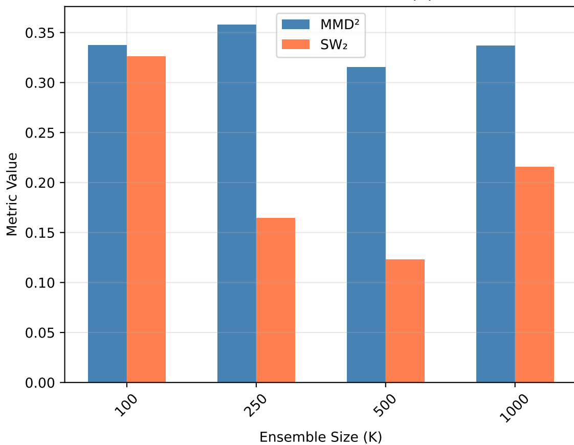
Ablation: Ensemble Size (K)
