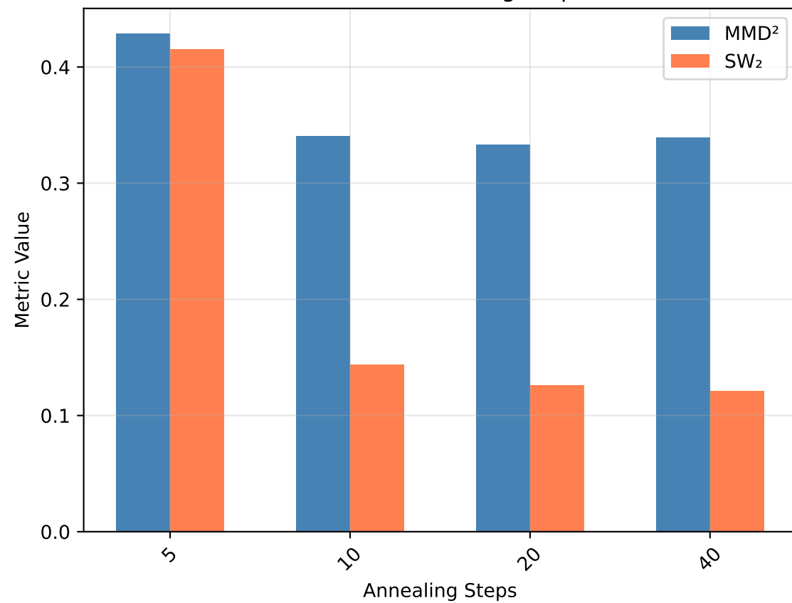
Ablation: Annealing Steps
