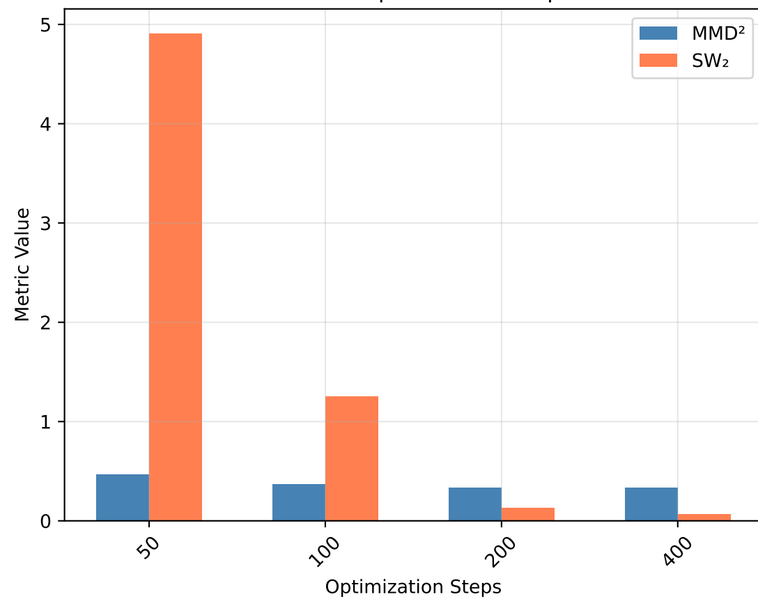
Ablation: Optimization Steps
