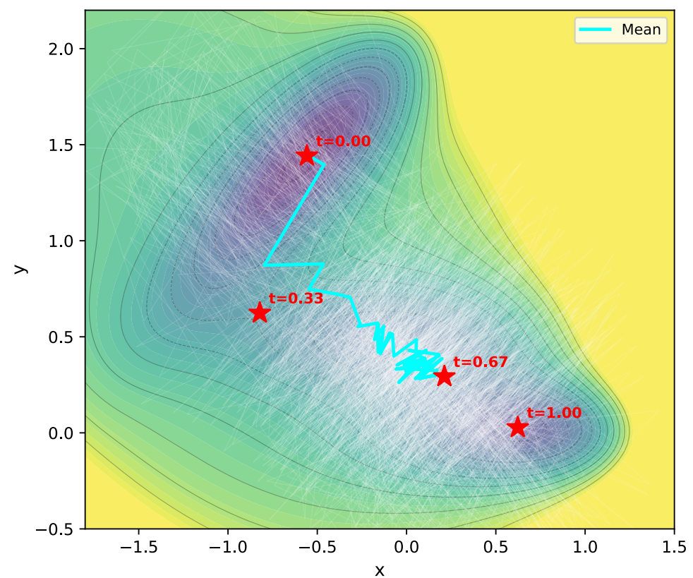
Vanilla SPDE (Eq. 6)
