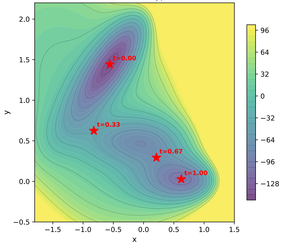
Müller-Brown V(x,y) & observation waypoints
