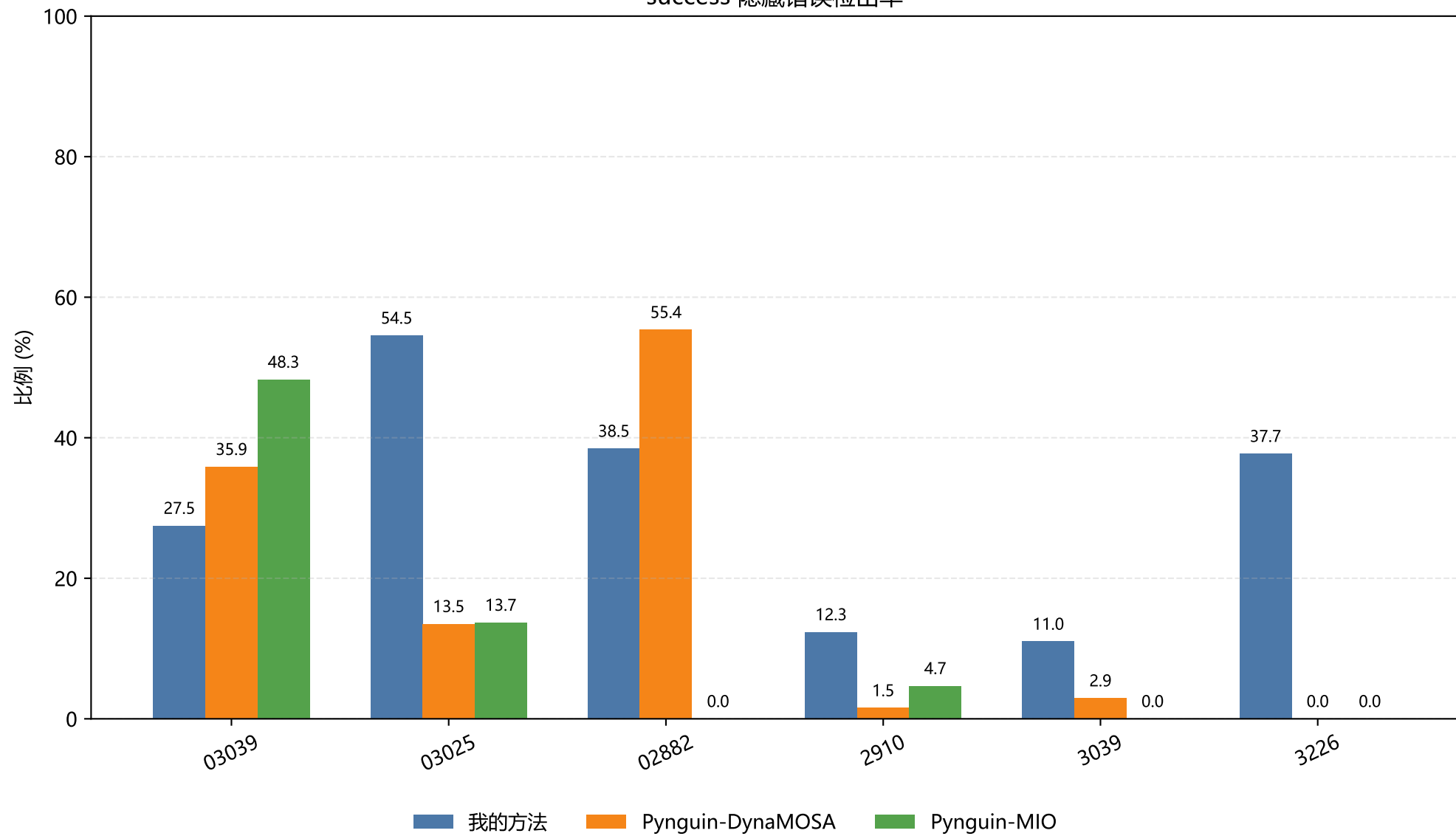
success 隐藏错误检出率
