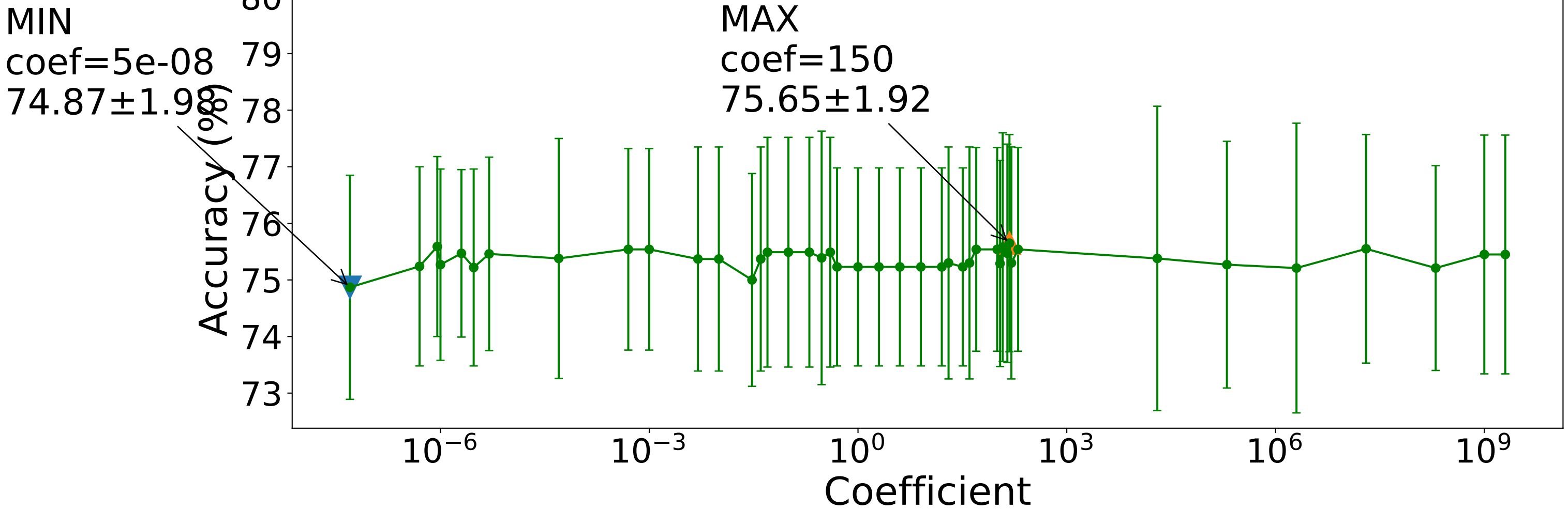
Squirrel: Accuracy vs Coefficient (mean \pm std)
