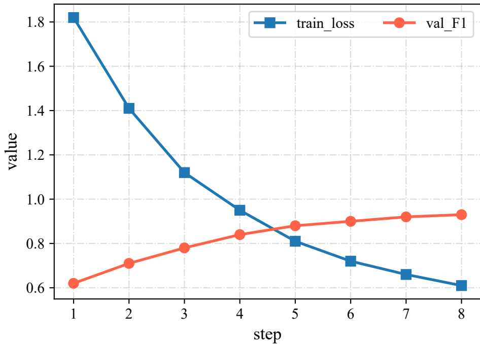
train loss and val F1 curves
