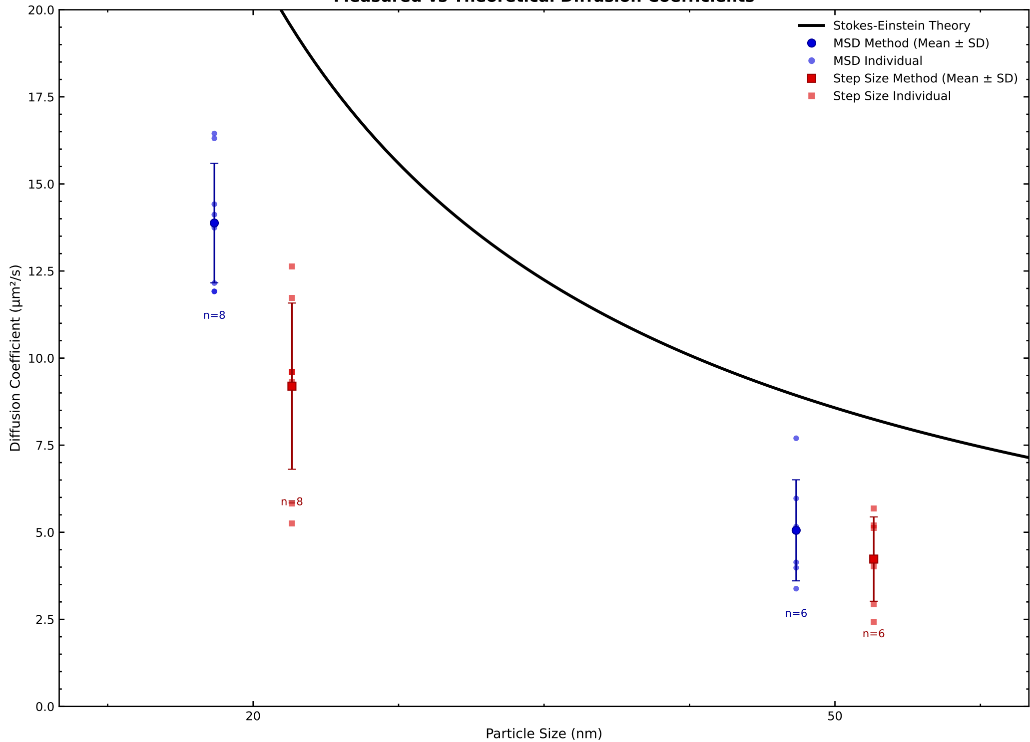
Measured vs Theoretical Diffusion Coefficients
