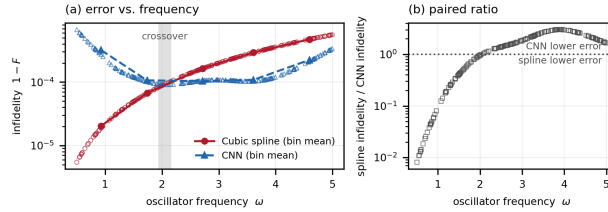
Figure 1: (a) Infidelity against \omega for spline and network on the 200 matched samples (open markers) with bin means, log ordinate; the curves cross near \omega \approx 2 (shaded). (b) Per-sample ratio of spline to network infidelity, crossing unity at the same transition.
