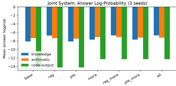
Figure 3. Joint system answer log-probability.
