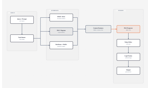
Figure 5. System architecture. The frozen backbone, RAG, and PLE memory provide three complementary evidence channels; the PLE Projector and token policy control logit-level fusion.
