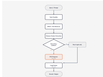
Figure 6. Inference pipeline. The token policy decides whether to apply the learned PLE Projector or bypass it with base logits only.
