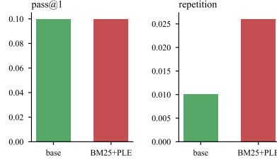
Figure 7. HumanEval pass@1 and mean repetition rate over 50 problems.
