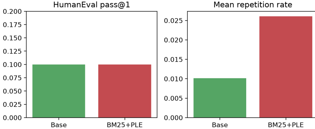
Figure 1: HumanEval 20: pass@1 and repetition rate.
