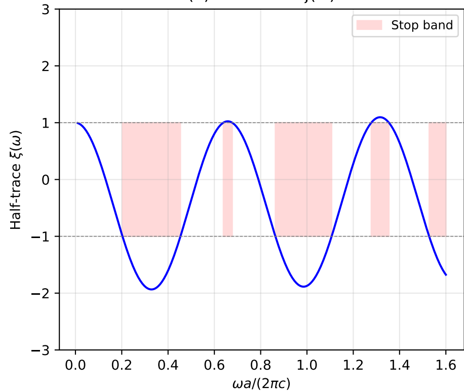
(a) Half-trace \xi(\omega)
