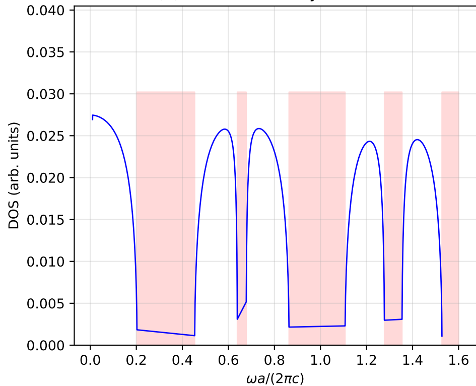
(b) Photonic density of states
