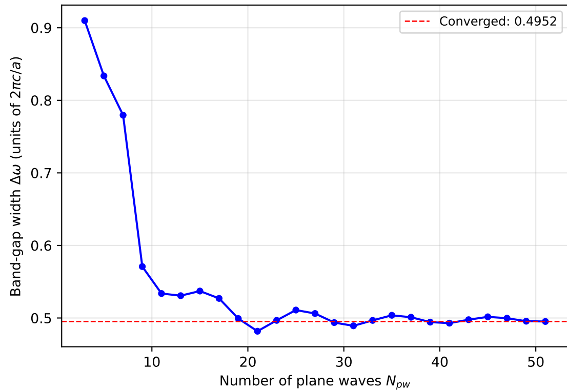
PWE convergence: 1D PhC ( \epsilon_a = 13 , \epsilon_b = 1 , f = 0.2 )
