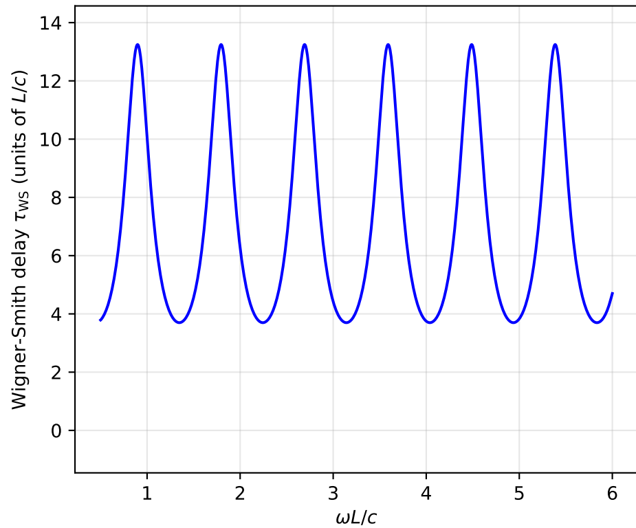
(b) Wigner-Smith time delay
