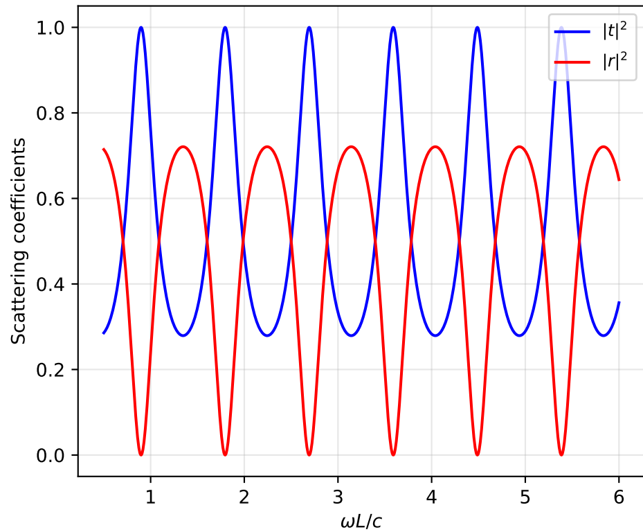
(a) Fabry-Perot transmission and reflection
