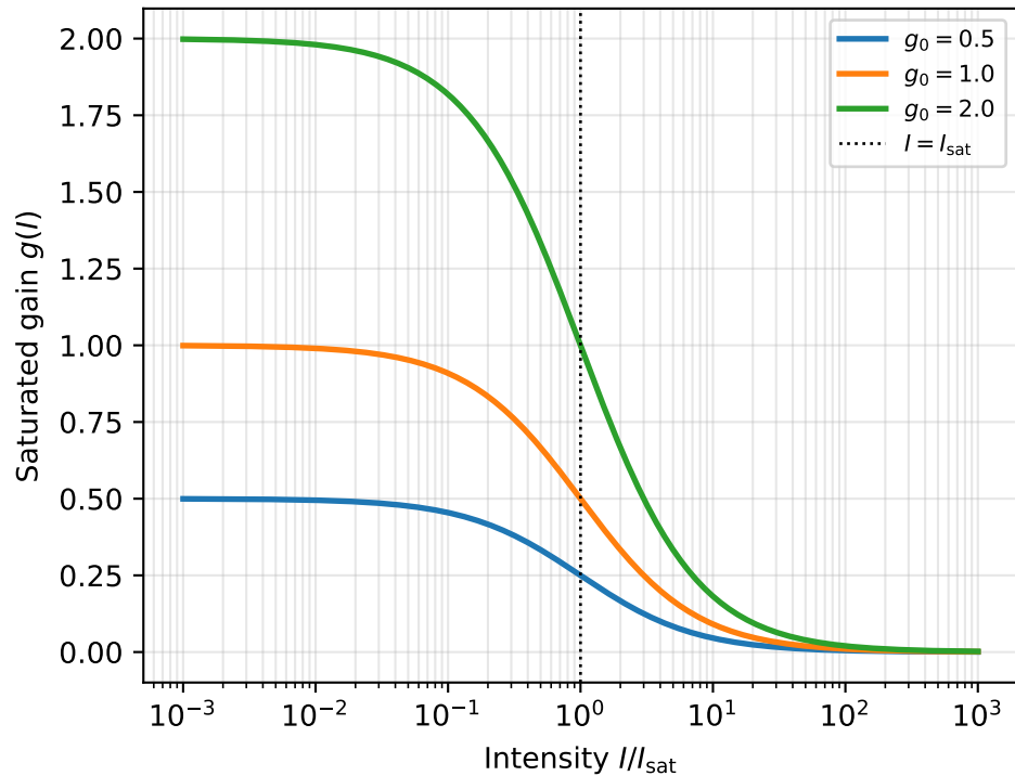
(a) Gain saturation g = g_0/(1 + I/I_{\text{sat}})
