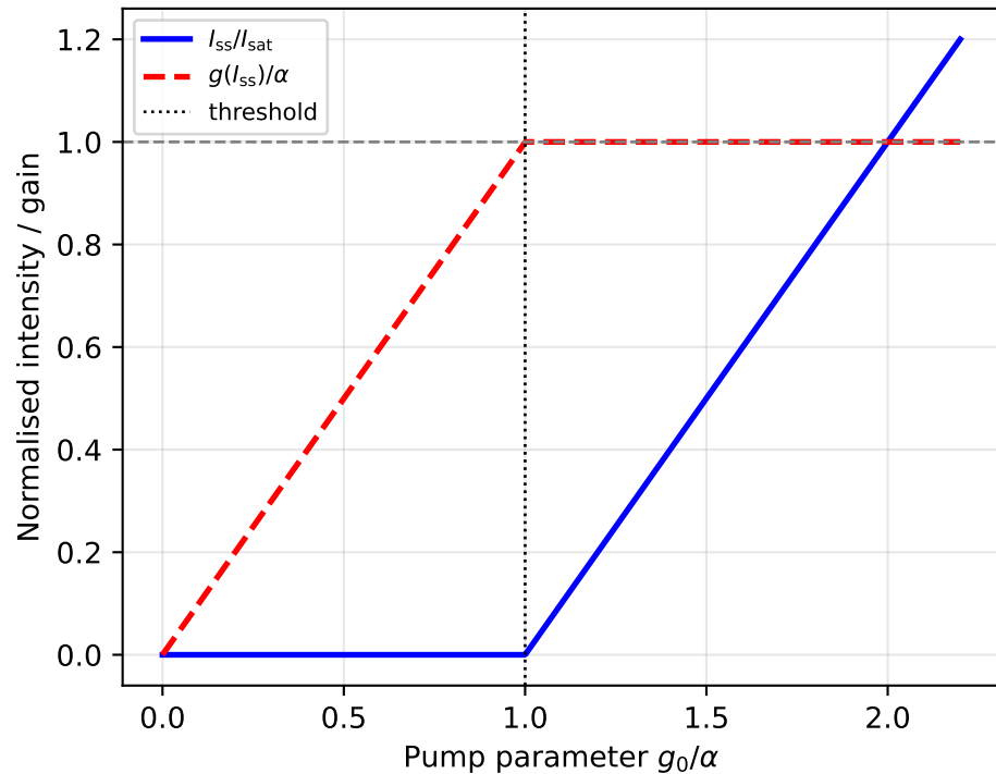
(b) Gain clamping above threshold
