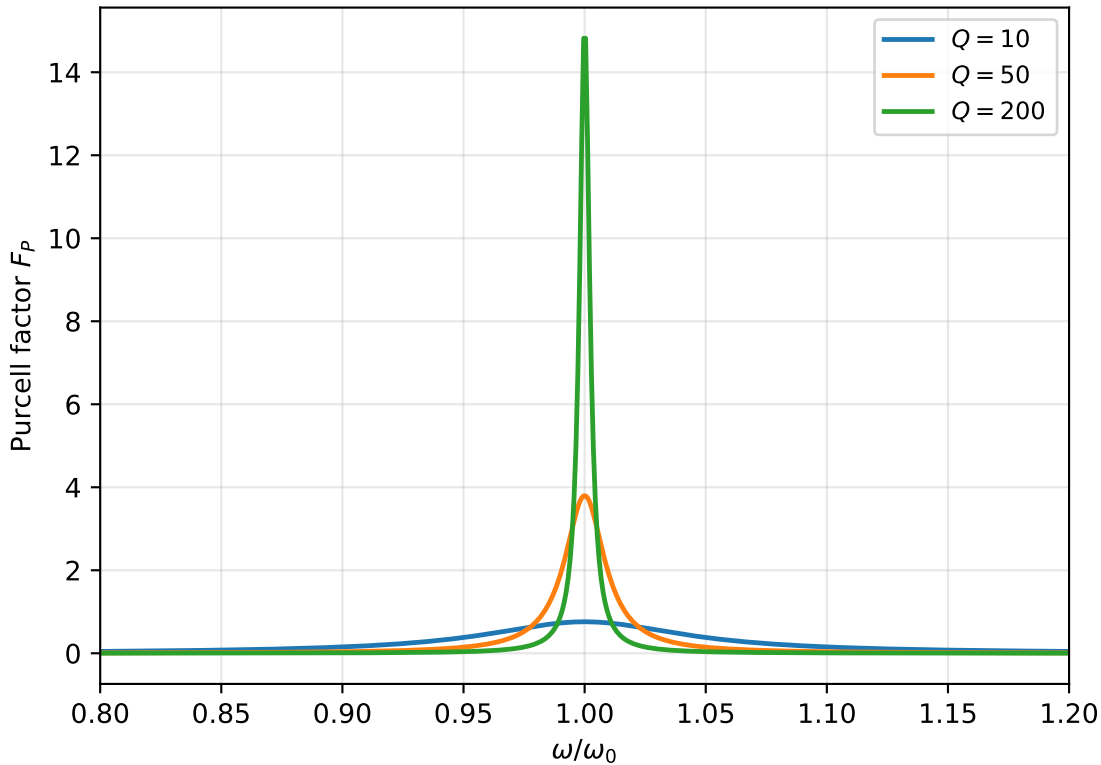
QNM Purcell enhancement near a lossy resonance
