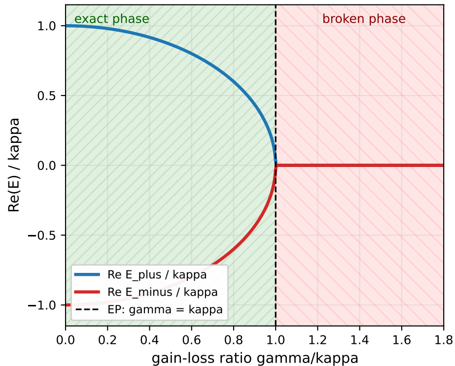
(a) Real eigenfrequency splitting
